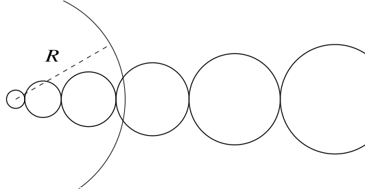
FIGURE 1. The set of Example 5.2 when r_i \nearrow +\infty . The relevant torsion function is in L_{loc}^{\infty}(\Omega) \setminus L^{\infty}(\Omega) and \lambda_{p,p}(\Omega) = 0 .
