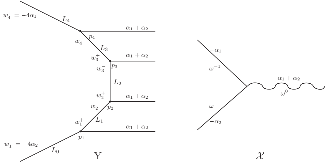
Figure 6. The toric web diagrams for Y and \mathcal{X} for n \geq 3 . Fixed points and invariants lines are labelled, together with the relevant torus and representation weights.
